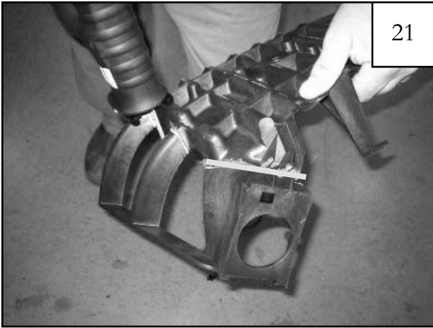
Using a hacksaw or saws all, carefully cut along lines made in Steps 19 and 20 to remove from portion of factory inner structure. Retain rearward piece.
