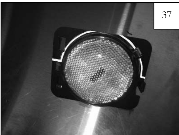
Carefully cut or grind factory light bezel along lines shown. Take care not to cut light lens.
